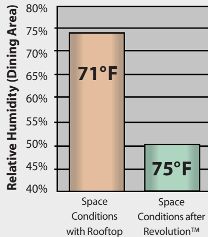
Figure 1: At a DOE sponsored restaurant pilot site, the owner/operator was able to raise the space thermostat by four degrees after installing Revolution™ to control space humidity. This improved comfort and reduced cooling energy costs by 30%.
